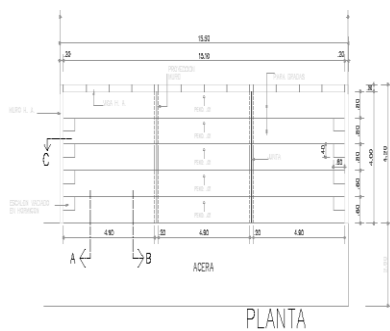
DETALLES CANCHA BASKETBALL 1:75
