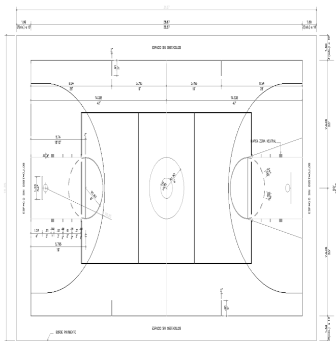
DETALLES CANCHA BASKETBALL 1:75
